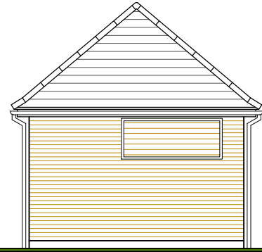
Side Elevation
